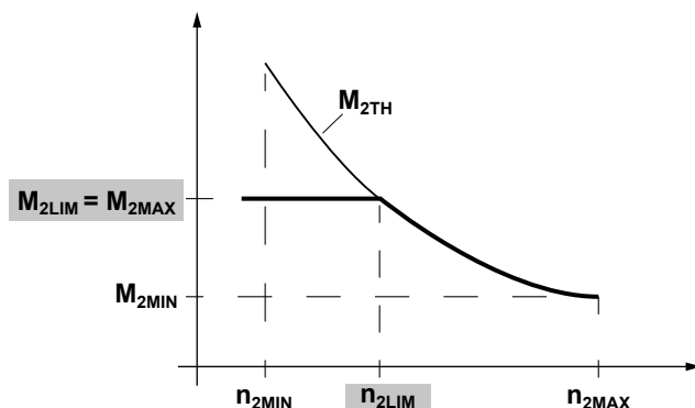
CURVA CARATTERISTICA / CHARACTERISTIC CURVE
